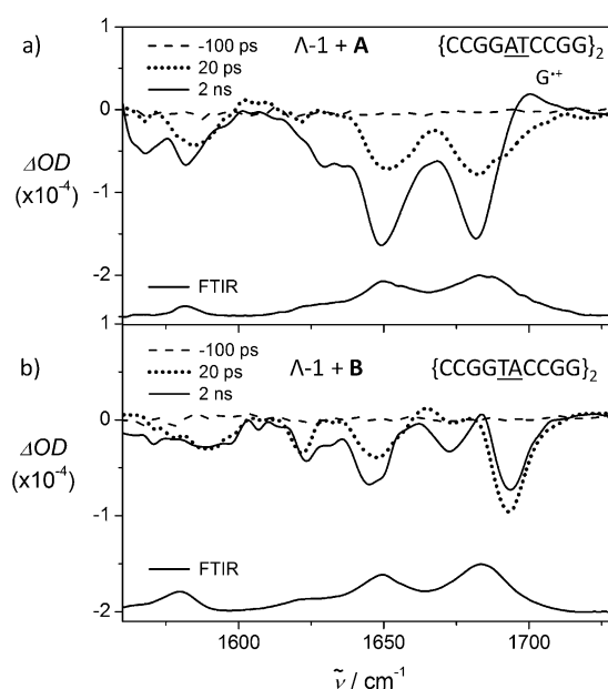
Figure 3. TRIR spectra of \Lambda -[Ru(TAP) 2 (dppz)] 2+ bound to a) {CCGGATCCGG} 2 and b) {CCGGTACCGG} 2 at selected delays. [Ru] = 400 \mu M, [ODN] = 500 \mu M in 50 mM phosphate-buffered D 2 O. \lambda_{\text{exc}} = 400 nm (100 fs, 1 \mu J). A baseline adjustment has been applied to the spectra. ODN FTIRs are also shown.
